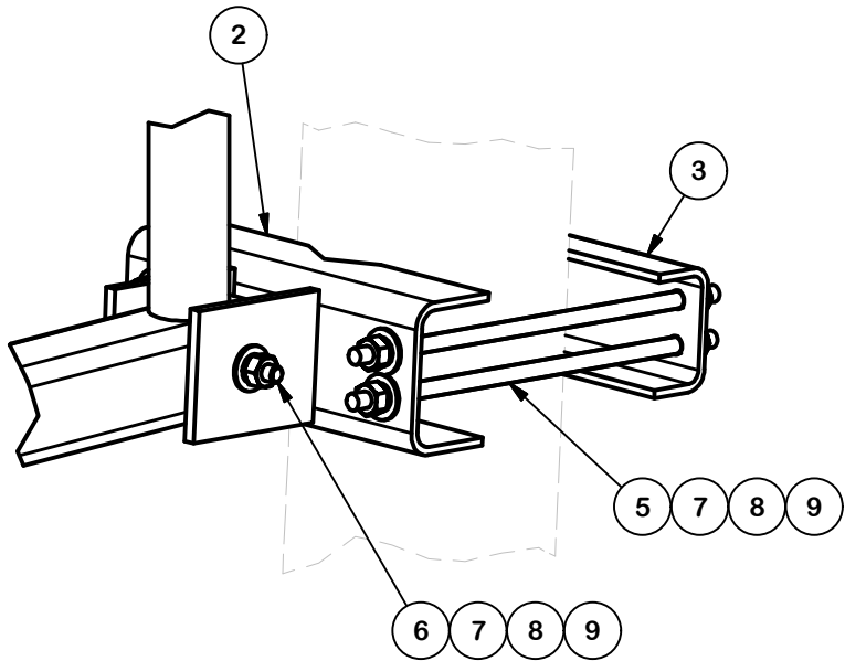
DETAIL B
